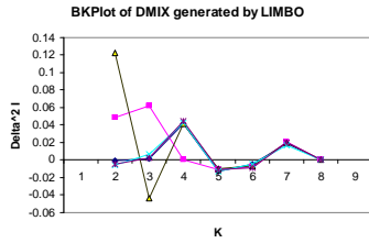
Fig. 30. BKPlots of DMIX data by LIMBO
