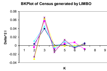
Fig. 31. BKPlots of Census data by LIMBO
