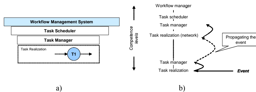
Figure 2. METEOR model competence hierarchy
