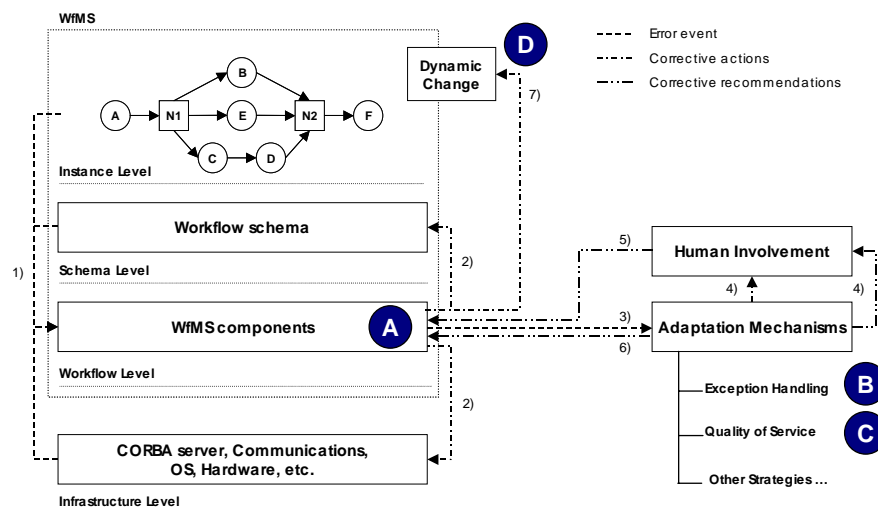
Figure 1. Adaptation architecture for WfMS
