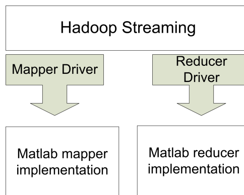
Figure 2. Using a driver to redirect input and output to Matlab implementations
