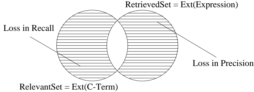
Figure 1: The mismatch between the RetrievedSet and Relevant Set
