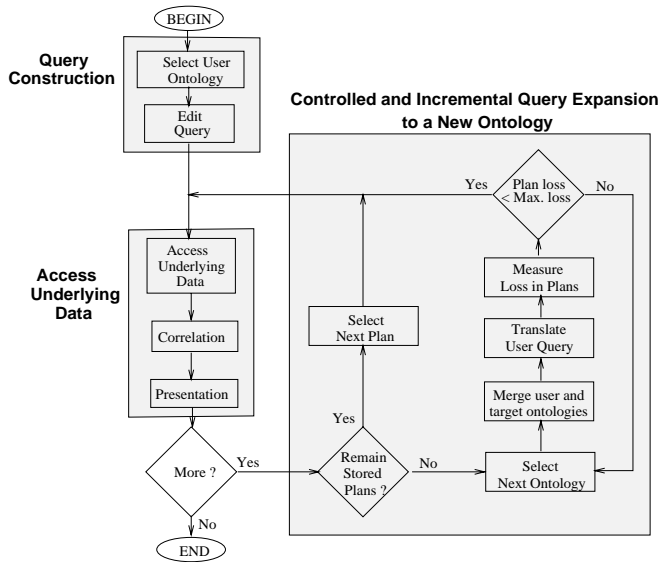
Figure 3: Detailed Query Processing in OBSERVER
