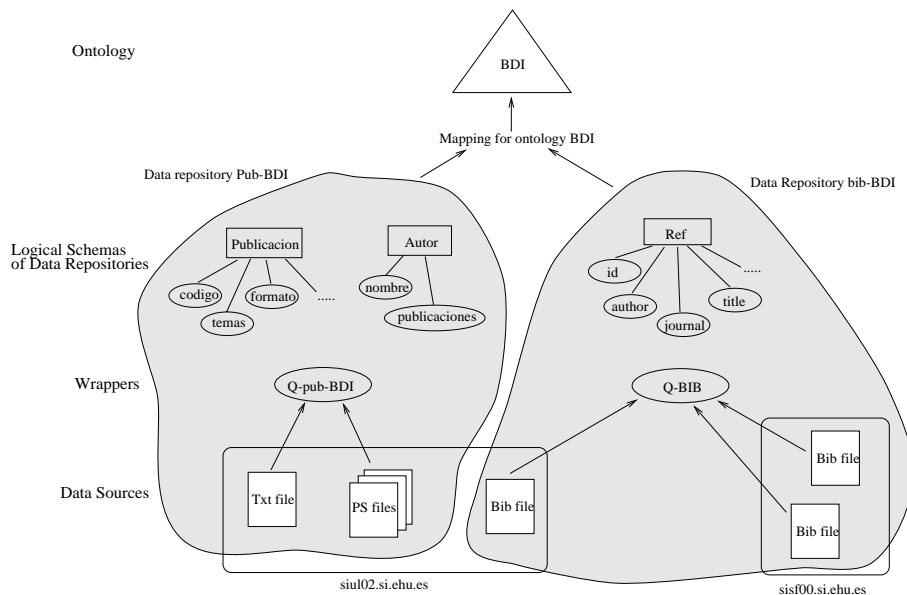
Figure 1: Data repositories, wrappers and data sources for ontology BDI
