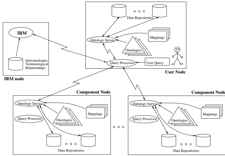
Figure 2: OBSERVER Global Architecture
