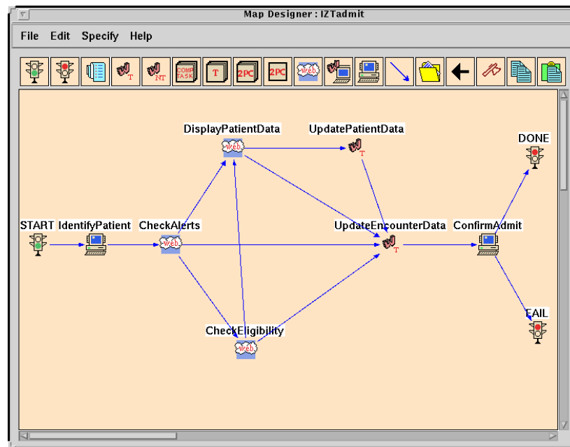
Figure 9. Admit Clerk Sub-Workflow Design
