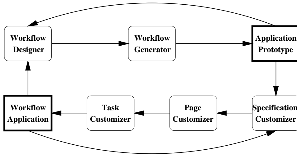
Figure 7. Rapid Workflow Application Development
