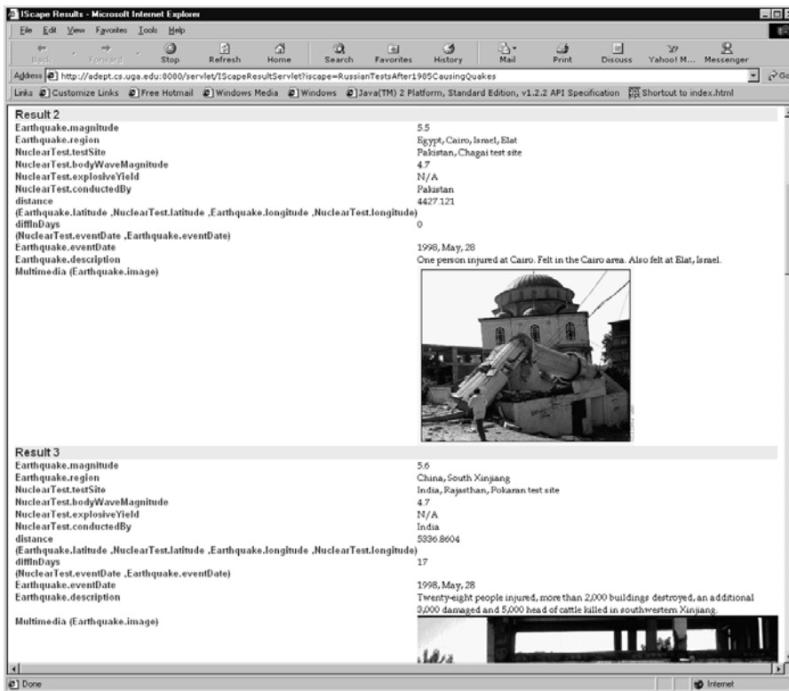
Fig. 16. Sample result page using Web interface to execute IScapes
