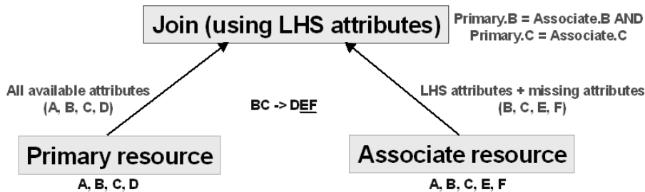
Fig. 6. Use of functional dependency to retrieve values for missing attributes
