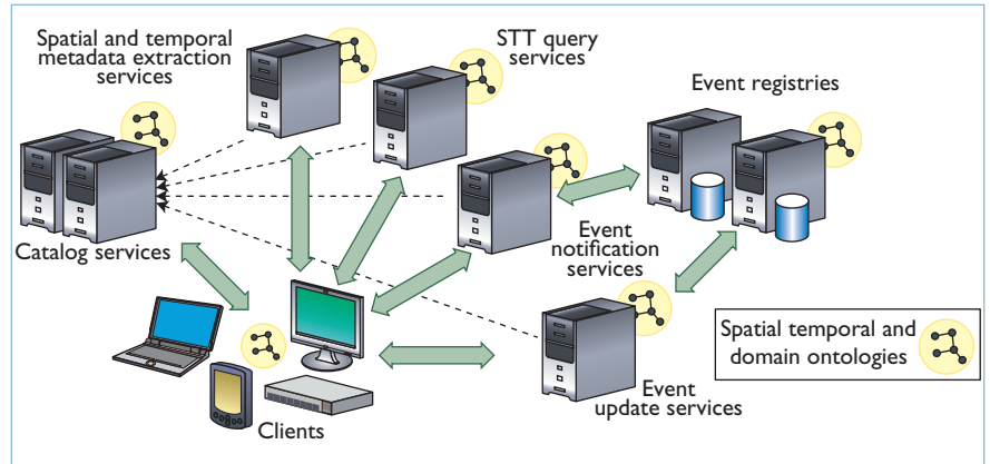
Figure 1. EventWeb architecture. The main components are event registries and various services for managing event data.
