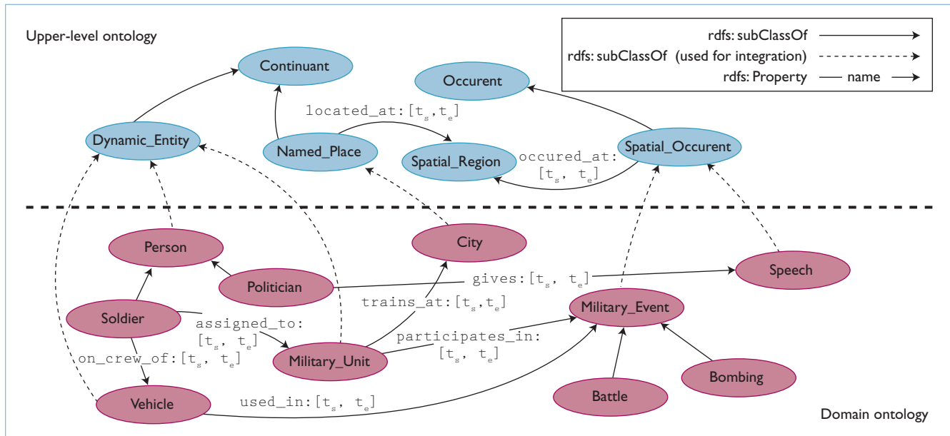
Figure 3. Ontology-based model of space, time, and theme. An upper-level ontology defining basic classes and relationships is shown in blue, and a sample military domain ontology is shown in magenta for illustration.
