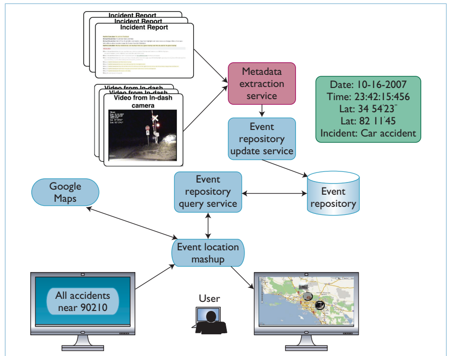
Figure 2. Example instantiation of the EventWeb architecture. A custom metadata extraction service extracts event-related spatial, temporal, and thematic (STT) metadata about police incidents from dashboard video and corresponding incident reports and loads the resulting events into an event repository. A client uses a query service in combination with Google Maps to create a mashup displaying all accidents near a specific area on a map.
