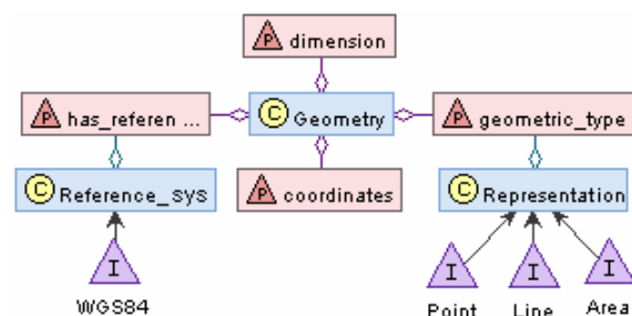
Figure 2. OGC Geometry model on RDF
