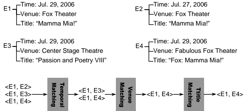
Figure 4. Illustration of an example for event disambiguation.
