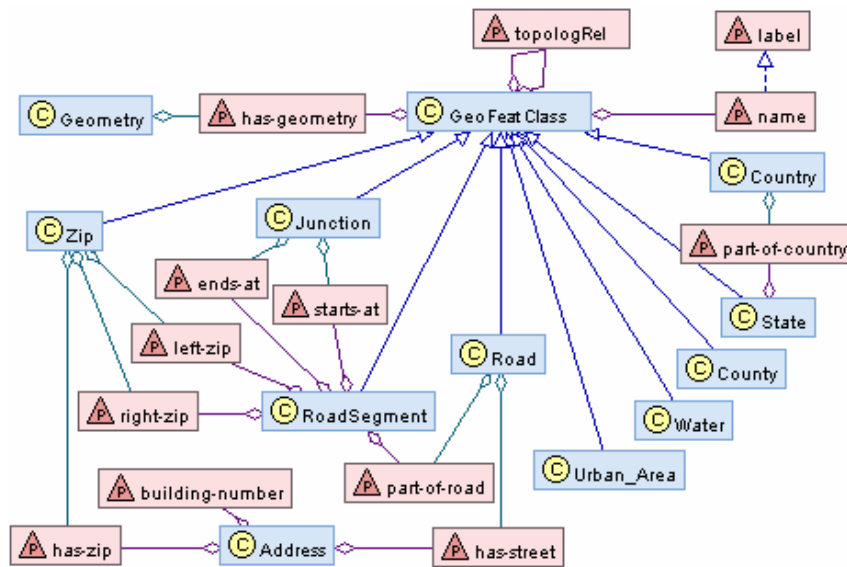
Figure 1. The RDF schema for geographic features. (C) and (P) denote RDF classes and properties, respectively
