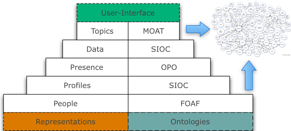
Figure 1: The SMOB Ontology stack
