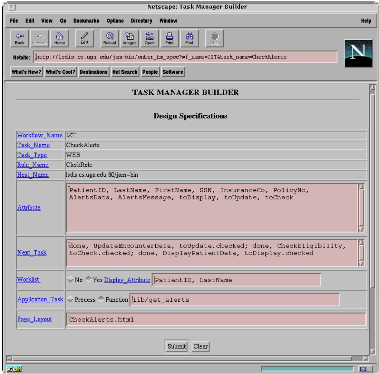
Figure 12: Check/Customize Task Specification
