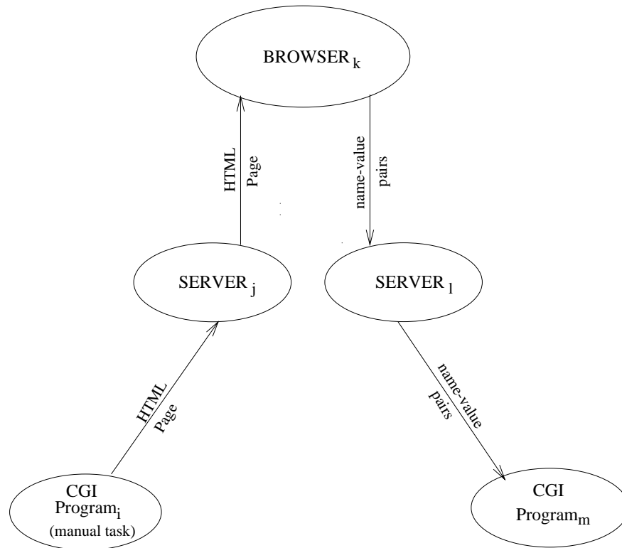
Figure 5: Invocation of Manual Tasks
