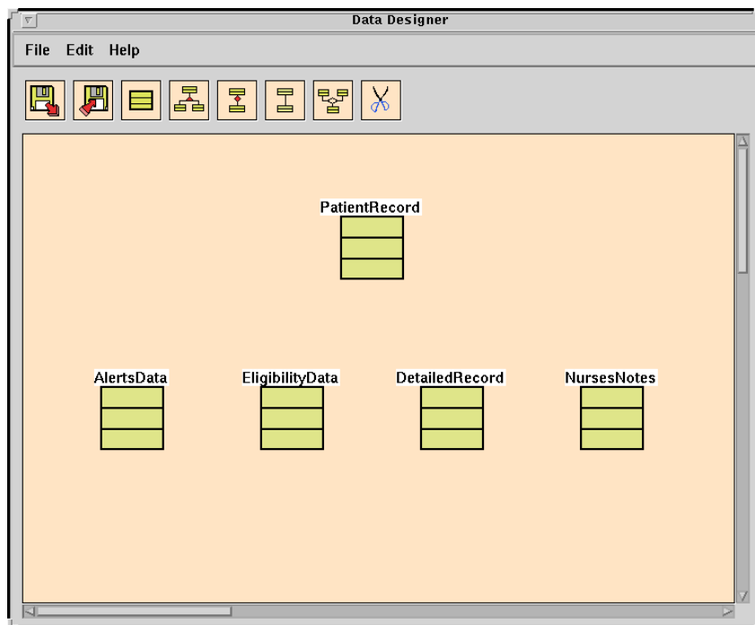
Figure 10: Immunization Tracking Data Design
