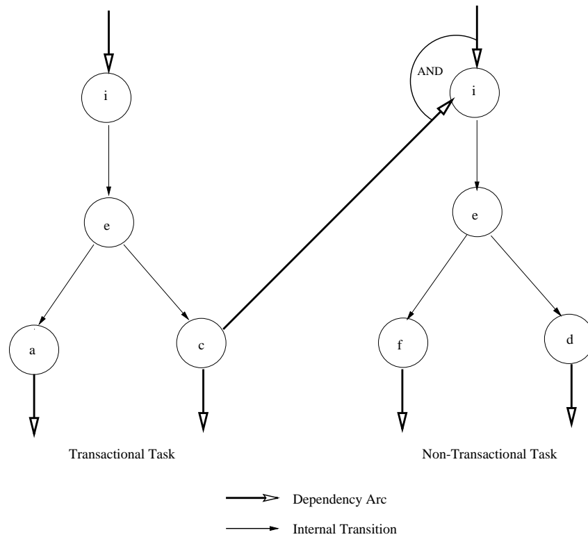
Figure 2: Task Structures
