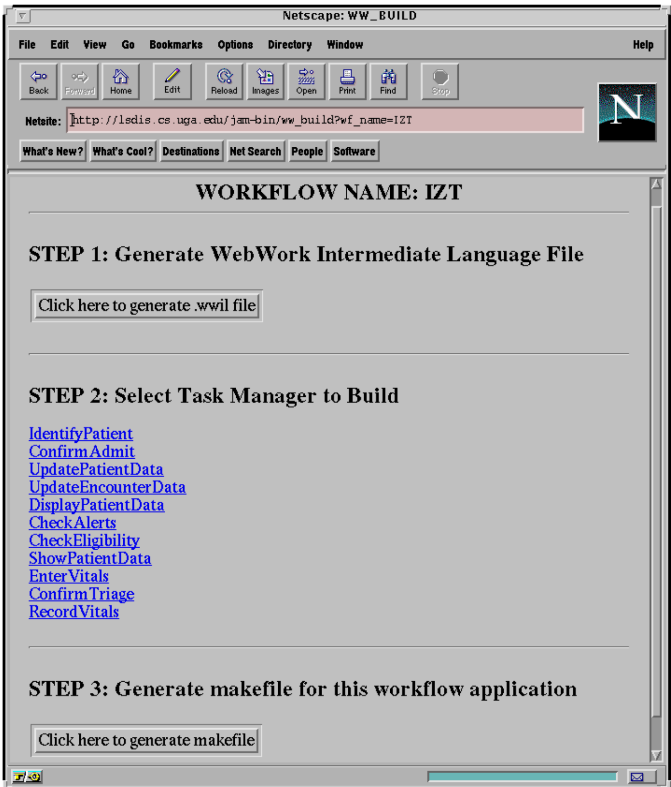
Figure 11: WebWork Builder
