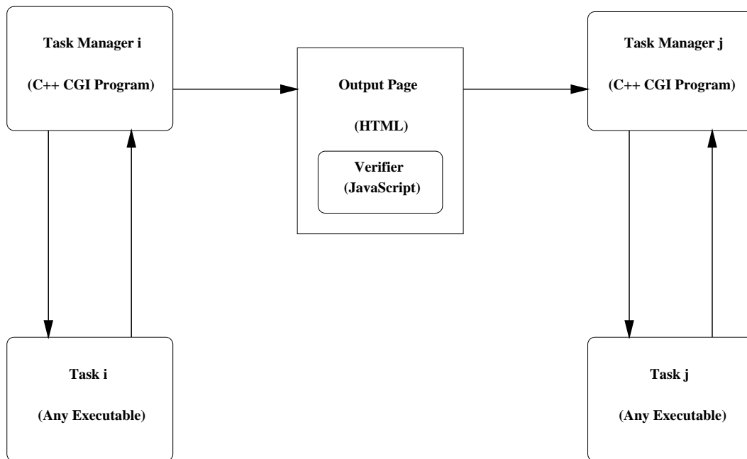
Figure 3: WebWork Execution Components
