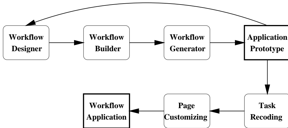
Figure 7: Rapid Workflow Application Development
