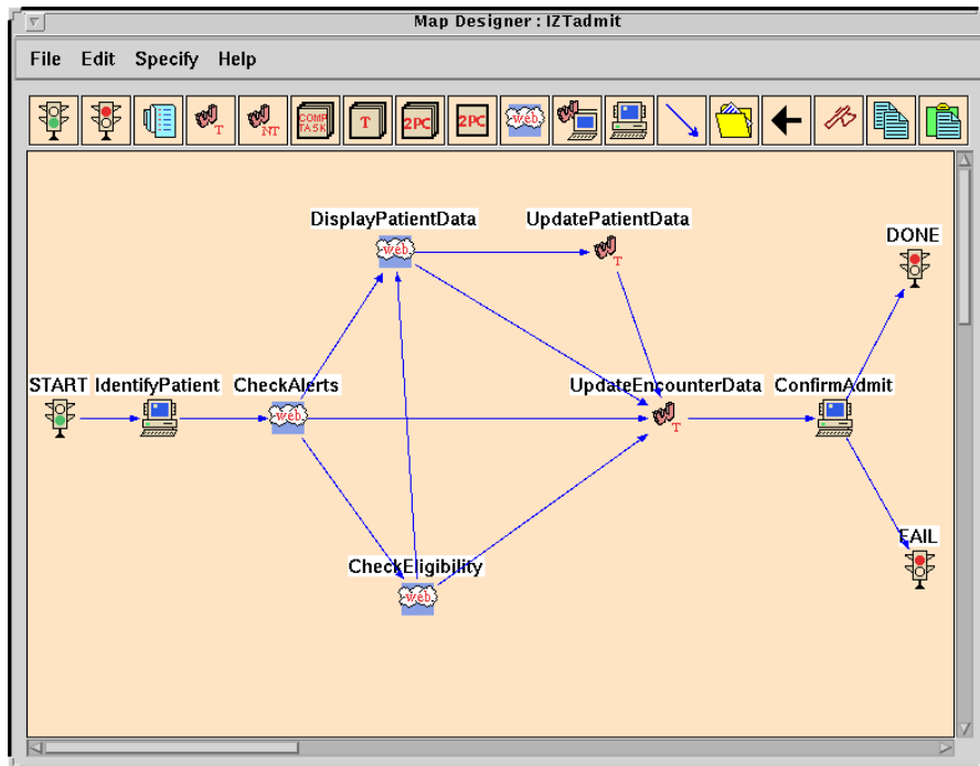
Figure 9: Admit Clerk Sub-Workflow Design
