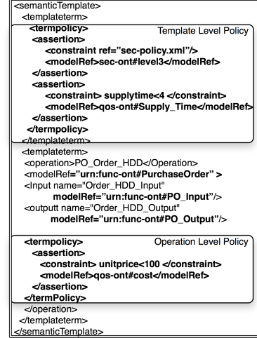
Figure 1. Semantic template modeling the requirements of the game manufacturer for ordering hard drives.
