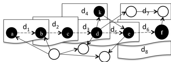
Figure 1. Document Reachability Framework
