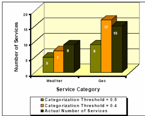
Fig. 1. Categorization statistics of Web services
