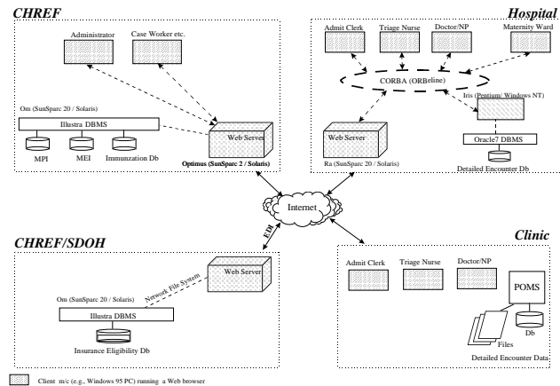
Figure 2: System Schematic
