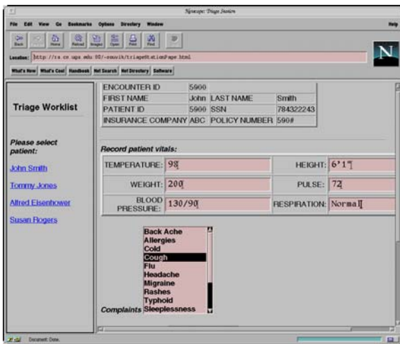
Figure 6: Triage Nurse's Interface
