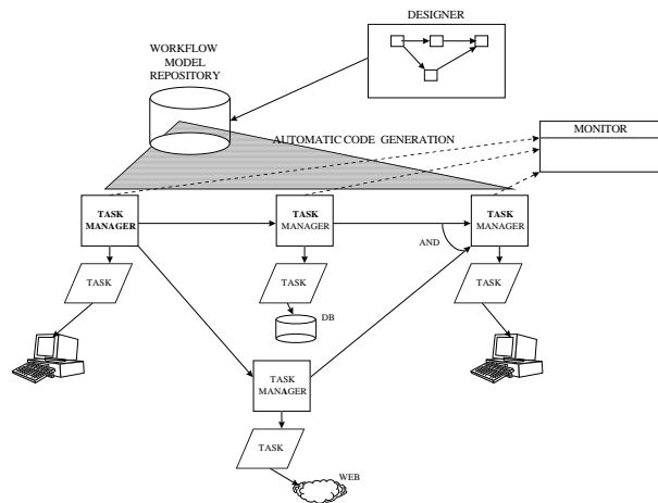
Figure 3: Meteor 2 Run-Time Model
