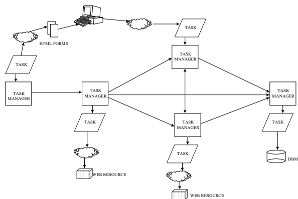
Figure 7: Distributed Architecture
